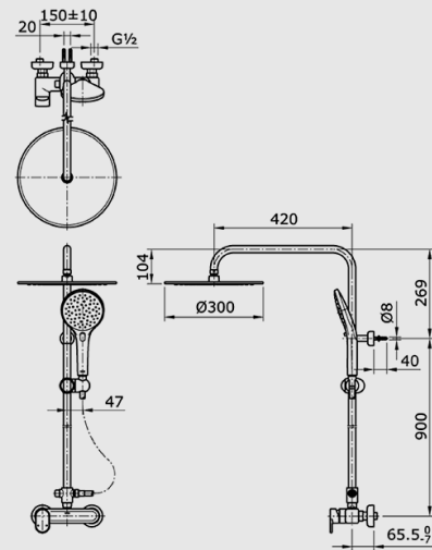
TX 492 MMC Shower Column Set
