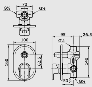
TX 442 MMC Single Lever Bath & Shower Mixer with Diverter
