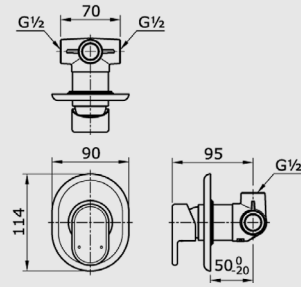
TX 443 MMC Single Lever Shower Mixer
