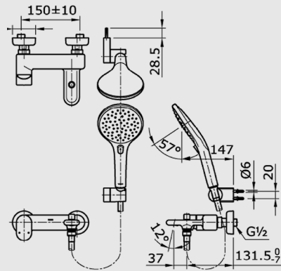
TX 471 MMC Single Lever Bath & Shower Set
