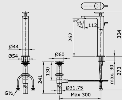
TX 116 MMC Extended Single Lever Lavatory Faucet with 1" Pop-Up Waste
