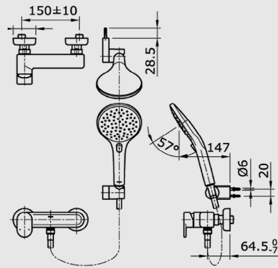
TX 474 MMC Single Lever Shower Set
