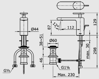
TX 115 MMC Single Lever Lavatory Faucet with 1 1/4" Pop-Up Waste
