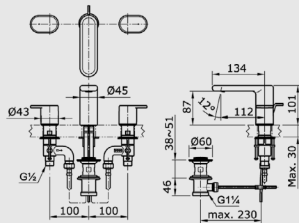
TX 119 MMC 8" Lavatory Faucet with 1 1/4" Pop-Up Waste
