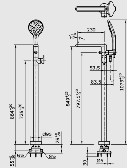
TX 494 MMC Floor Standing Bath & Shower Set
