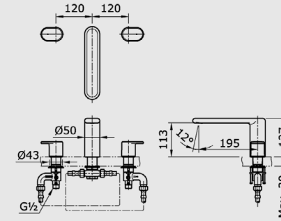
TX 467 MMC Bath Filler & Mixer
