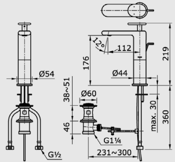
TX 116 MMC V4 Extended Single Lever Lavatory Faucet with 1 1/4" Pop-Up Waste
