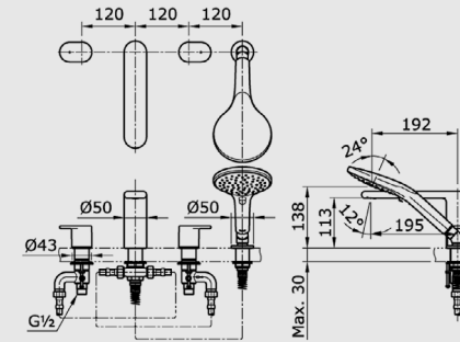
TX 447 MMC 4 Holes Bath & Shower Set
